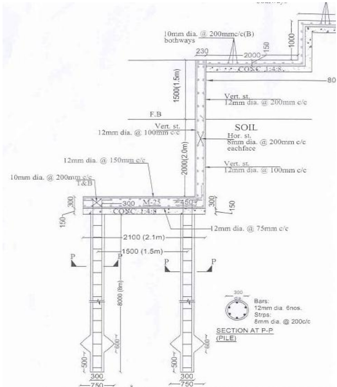
R.C.C. RETAINING WALL SECTION FOR 2m RETAINING OF SOIL
