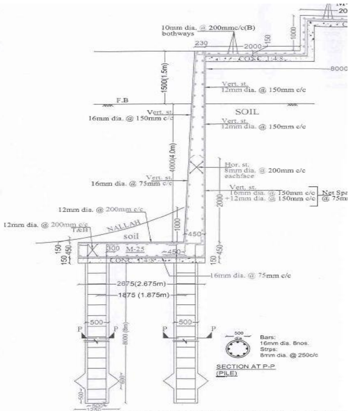
R.C.C. RETAINING WALL SECTION FOR 4m RETAIN
