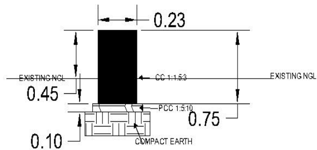
FOUNDATION DETAIL VERTICAL MEMBER OF 50 X 50 X 2.9 mm size
