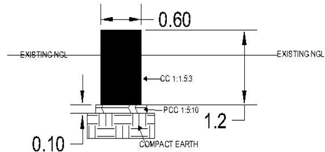
TYPICAL MAIN STRUCTURE MEMBER (96 X 50 MM) FOUNDATION DETAIL Dimensions are in metres
